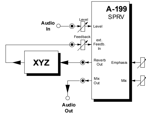
Fig. 3: External feedback
